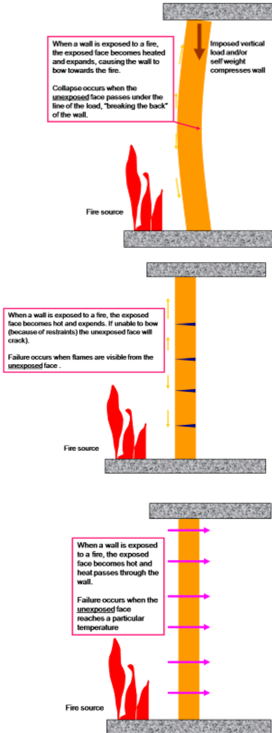
Fire Test to AS 1530.4
